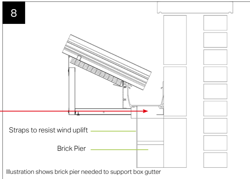
Illustration shows raised back box gutter
