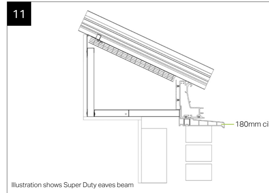
Illustration shows standard eaves beam
