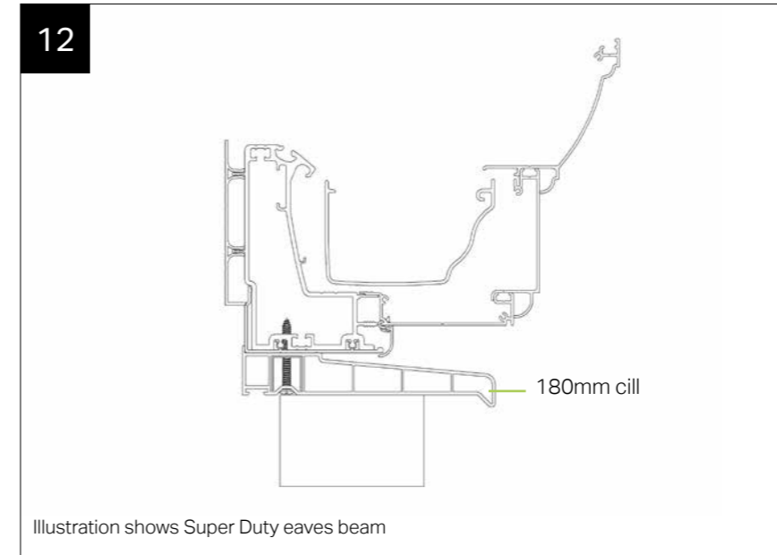
Illustration shows Super Duty eaves beam
