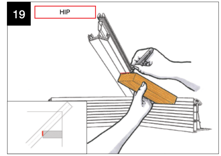
From the location plan, now mark the right hand fixing position.
