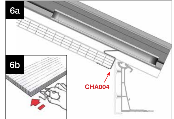
6a Attach CHA004 to the cloaking panel and fit as shown in the main internal insulated pelmet installation guide. (page 16). 6b
