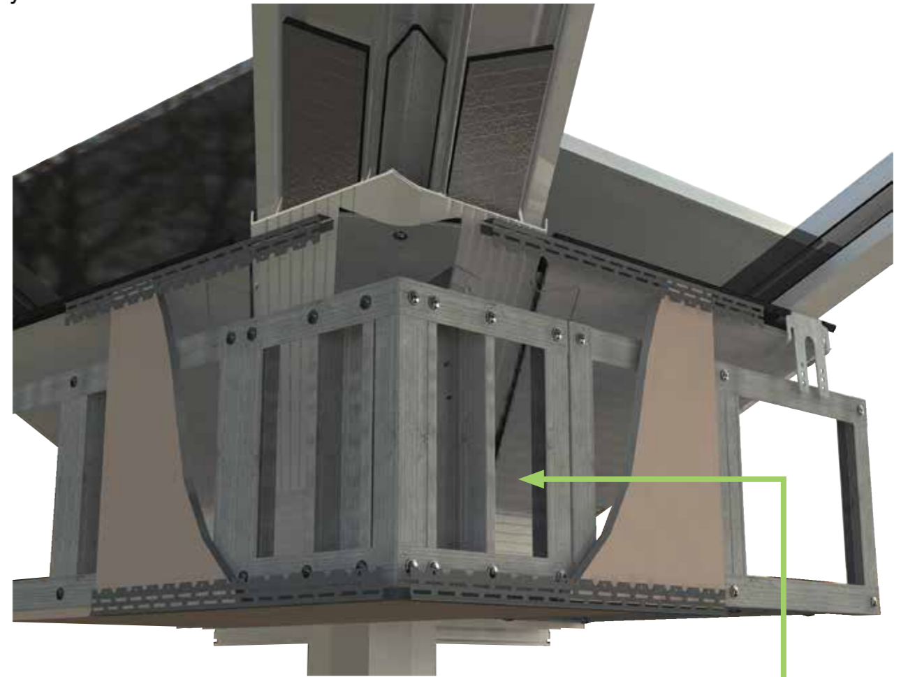
Valley Section
