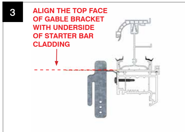
3 ALIGN THE TOP FACE OF GABLE BRACKET WITH UNDERSIDE OF STARTER BAR CLADDING Attach gable bracket to frame using two of the CHA008 (4.8 x 32mm) self drill Phillips Pan Head screws supplied.
