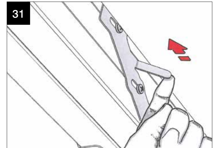
Fit the cloaking panel (silver side up) between the bolsters supported at the eaves by the support clips CHA002. Next bend back the long legged tabs on the CHA013 to hold the polycarbonate cloaking trim in its final position.
