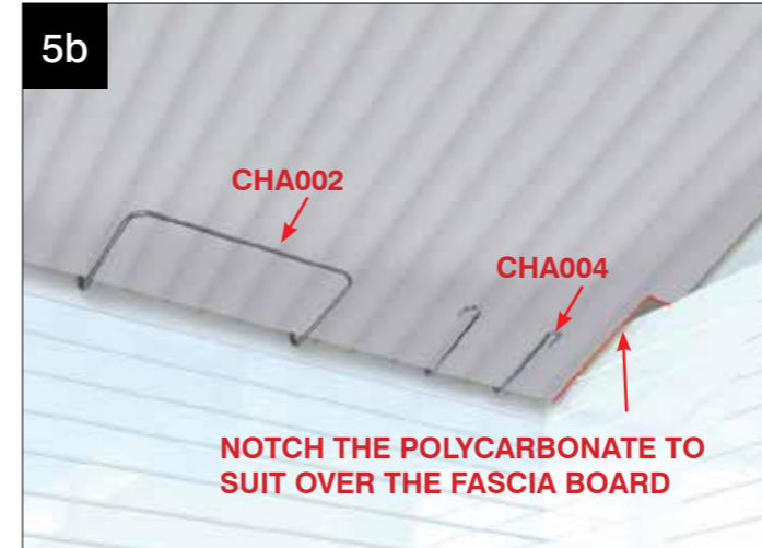
5b Referring to the location plan, take the appropriate piece of polycarbonate cloaking panel, mark and notch the corner as demonstrated.
