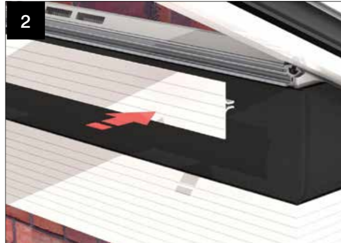
2 Fit length of LHE---/2 to the upper section of box gutter.
