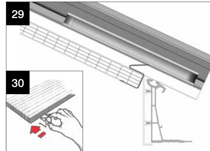
Now attach these polycarbonate support spacers CHA004 – attach to the leading edge of the polycarbonate (silver side up). Location plan and '●' symbol shows where they are fitted.
