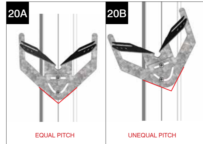
Now offer up the Georgian hip bracket (CHA090) – where the roof is equal pitch across the hip, the bracket should sit as (a). On unequal pitches, the bracket may be skewed as in (b)
