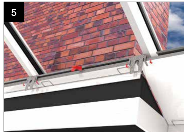
5 Fit the polycarbonate modesty panels and bend over bracket legs to secure.
